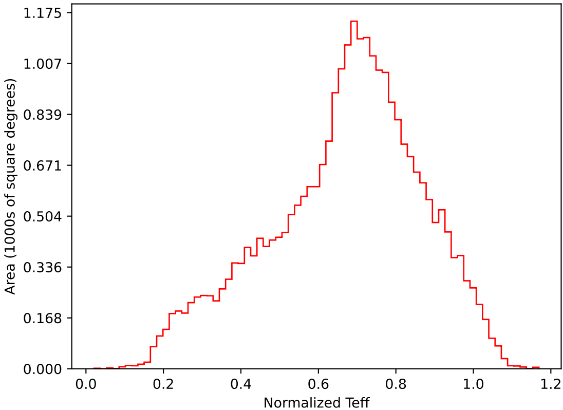
too_elab_r8_d2_griz_v3.4_10yrs All sky i band: Normalized Teff
