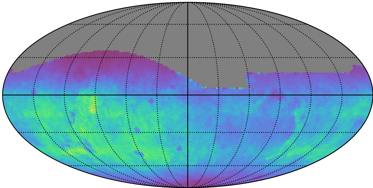
too_elab_r8_d2_griz_v3.4_10yrs All sky g band: Normalized Teff
