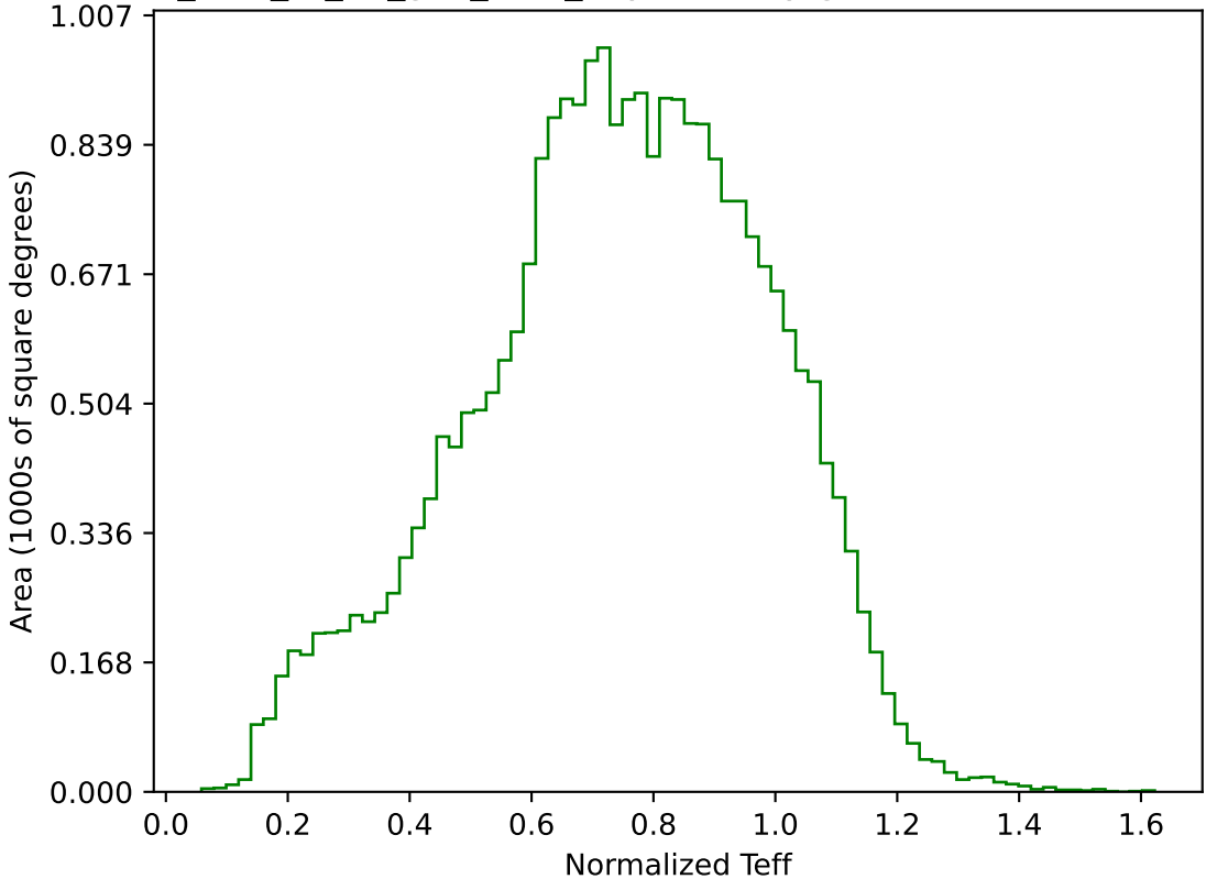
too_elab_r8_d2_griz_v3.4_10yrs All sky g band: Normalized Teff
