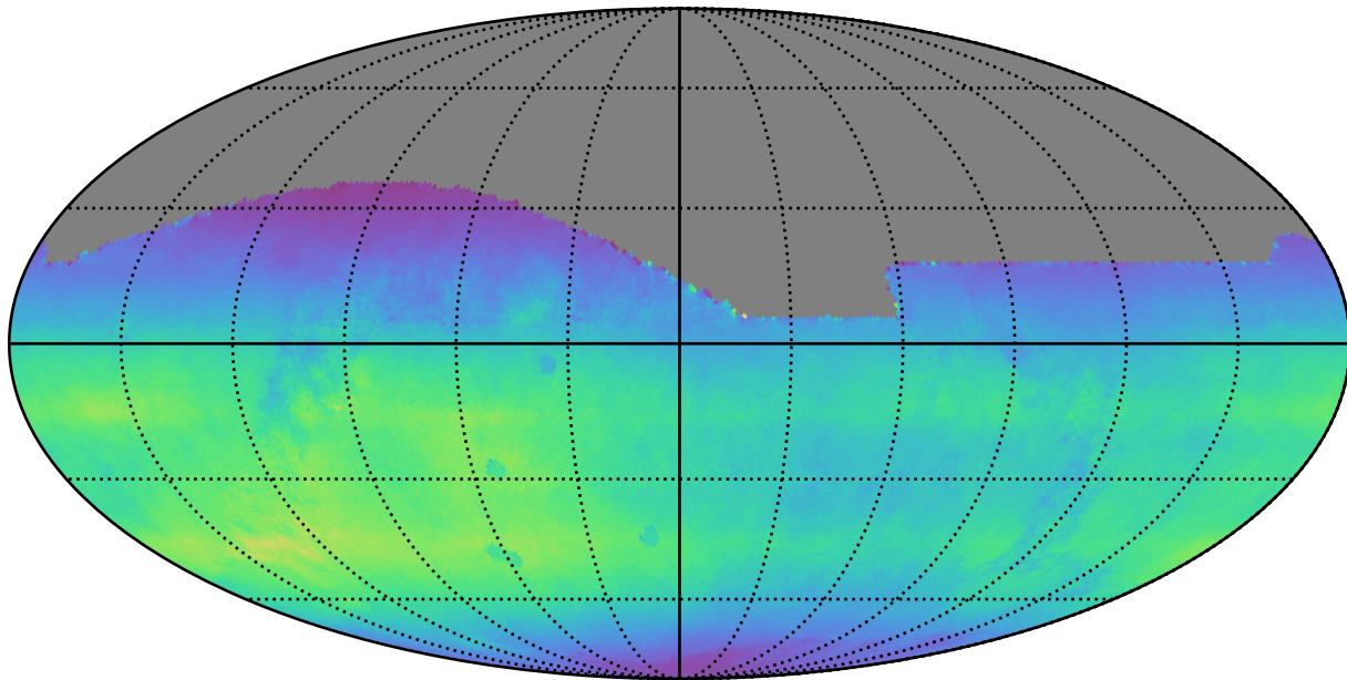
too_elab_r8_d2_griz_v3.4_10yrs All sky all bands: Normalized Teff
