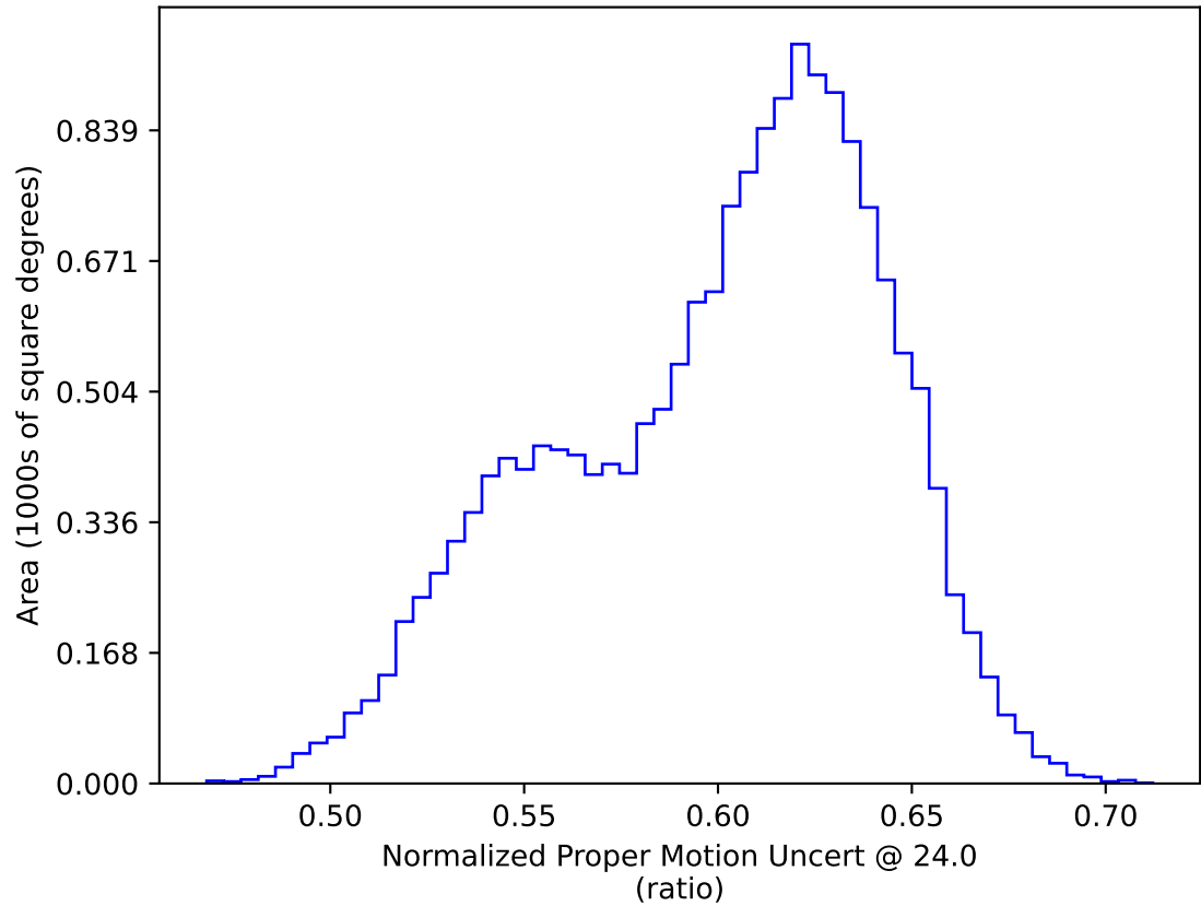
too_elab_r8_d2_griz_v3.4_10yrs WFD: Normalized Proper Motion Uncert @ 24.0
