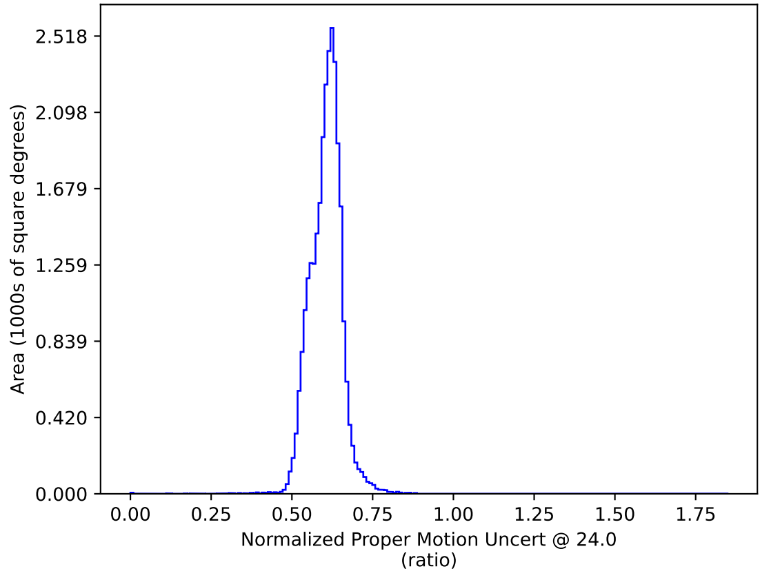
too_elab_r8_d2_griz_v3.4_10yrs All sky: Normalized Proper Motion Uncert @ 24.0
