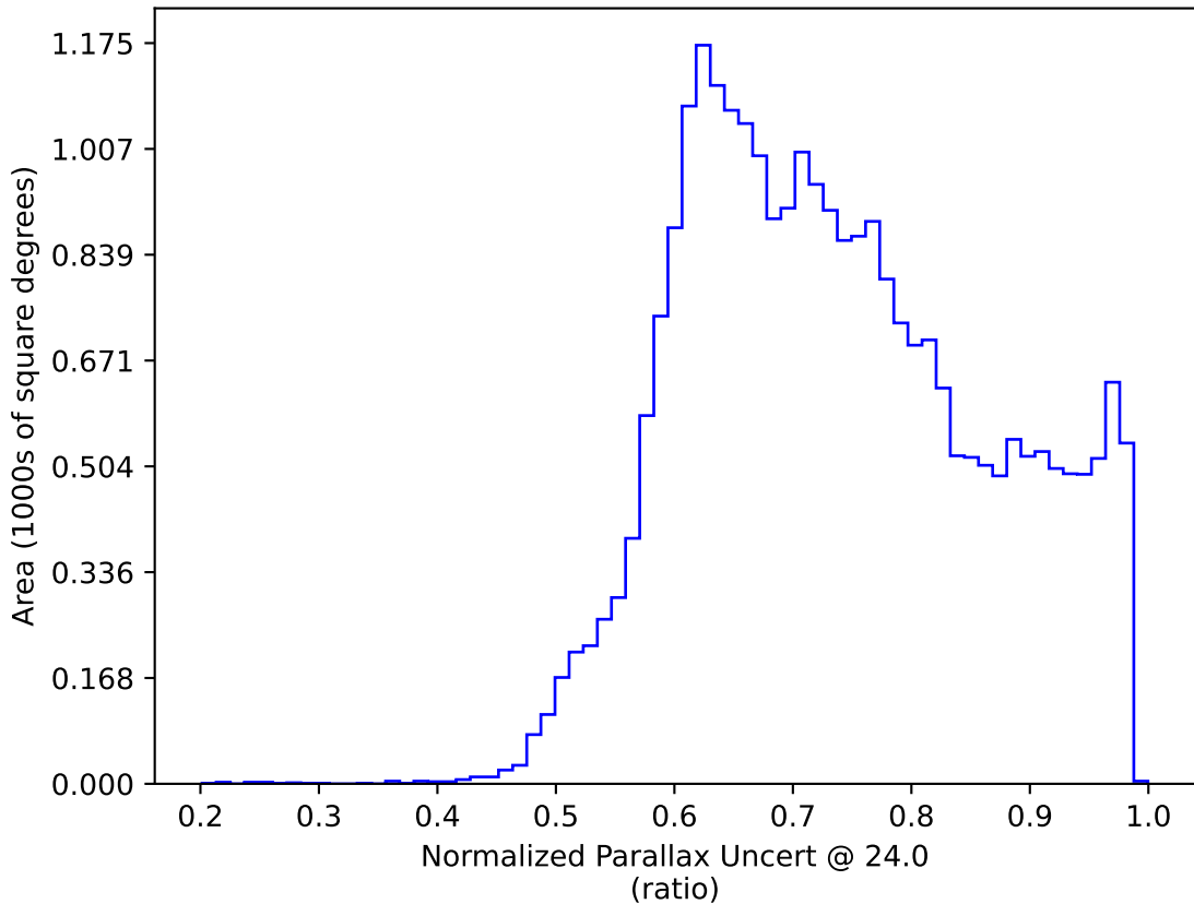
too_elab_r8_d2_griz_v3.4_10yrs All sky: Normalized Parallax Uncert @ 24.0
