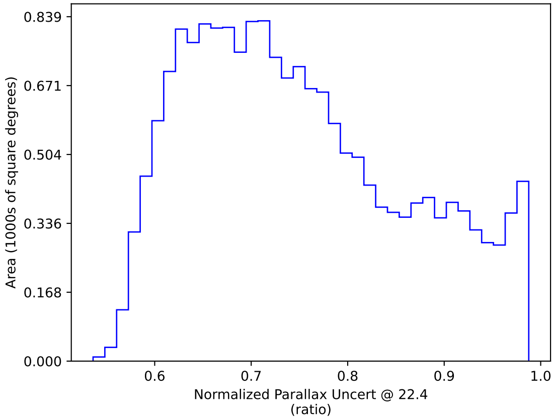
too_elab_r8_d2_griz_v3.4_10yrs WFD: Normalized Parallax Uncert @ 22.4
