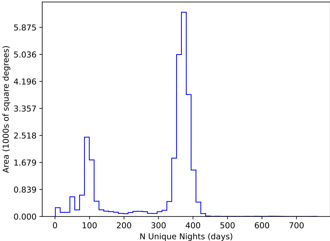
too_elab_r8_d2_griz_v3.4_10yrs All sky all bands: N Unique Nights
