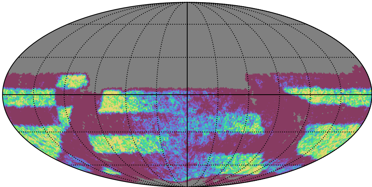
too_elab_r8_d2_griz_v3.4_10yrs Yr 3-4 y band: NVisits
