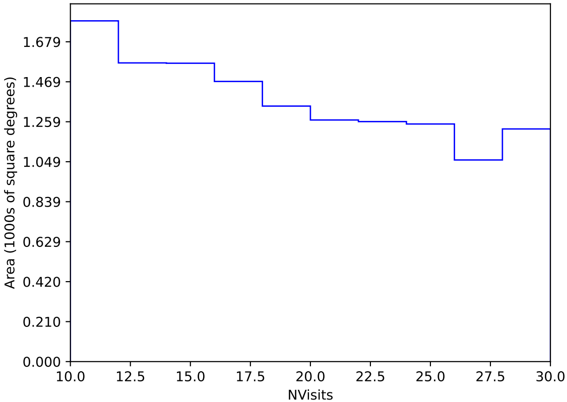
too_elab_r8_d2_griz_v3.4_10yrs Yr 3-4 y band: NVisits
