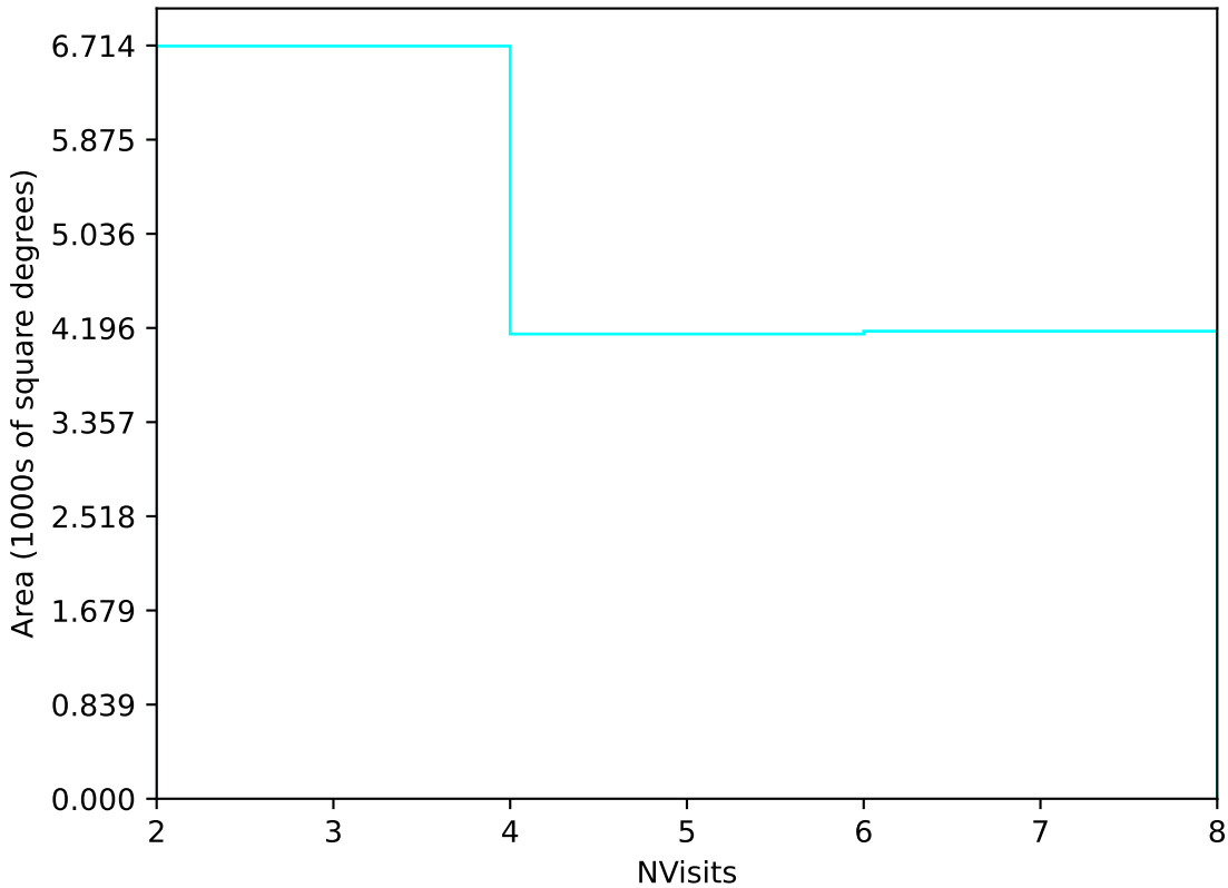
too_elab_r8_d2_griz_v3.4_10yrs Yr 3-4 u band: NVisits
