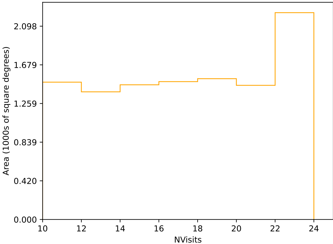
too_elab_r8_d2_griz_v3.4_10yrs Yr 3-4 r band: NVisits
