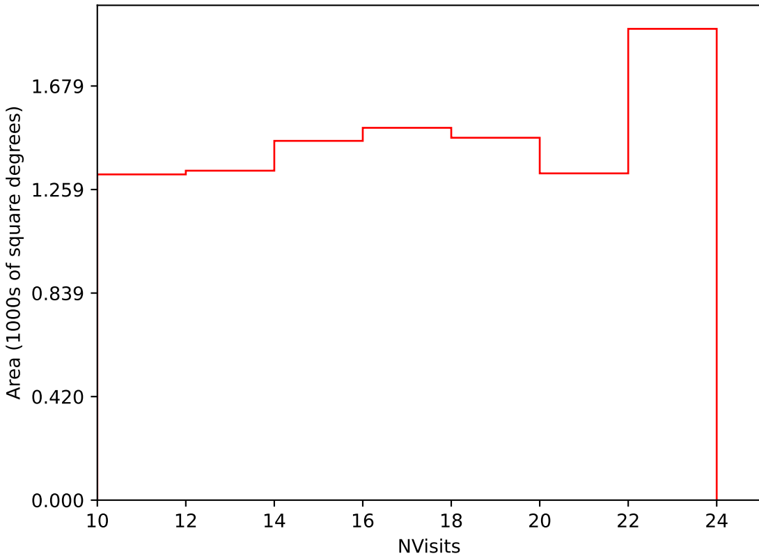
too_elab_r8_d2_griz_v3.4_10yrs Yr 3-4 i band: NVisits
