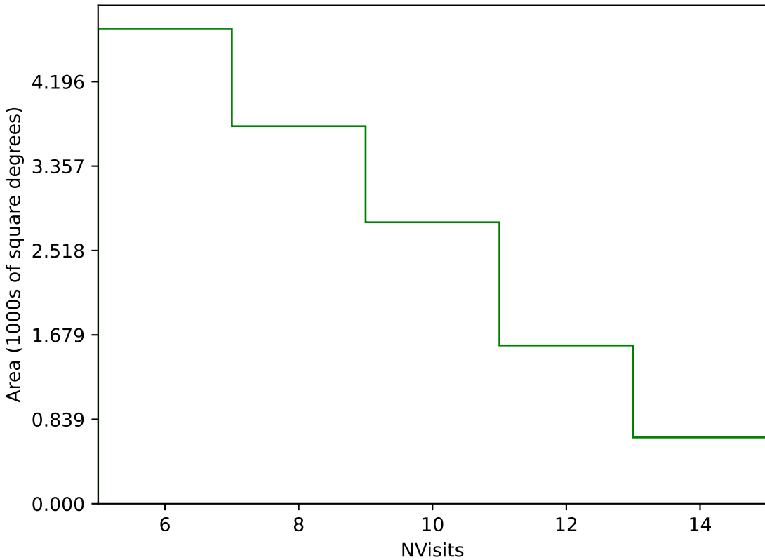
too_elab_r8_d2_griz_v3.4_10yrs Yr 3-4 g band: NVisits
