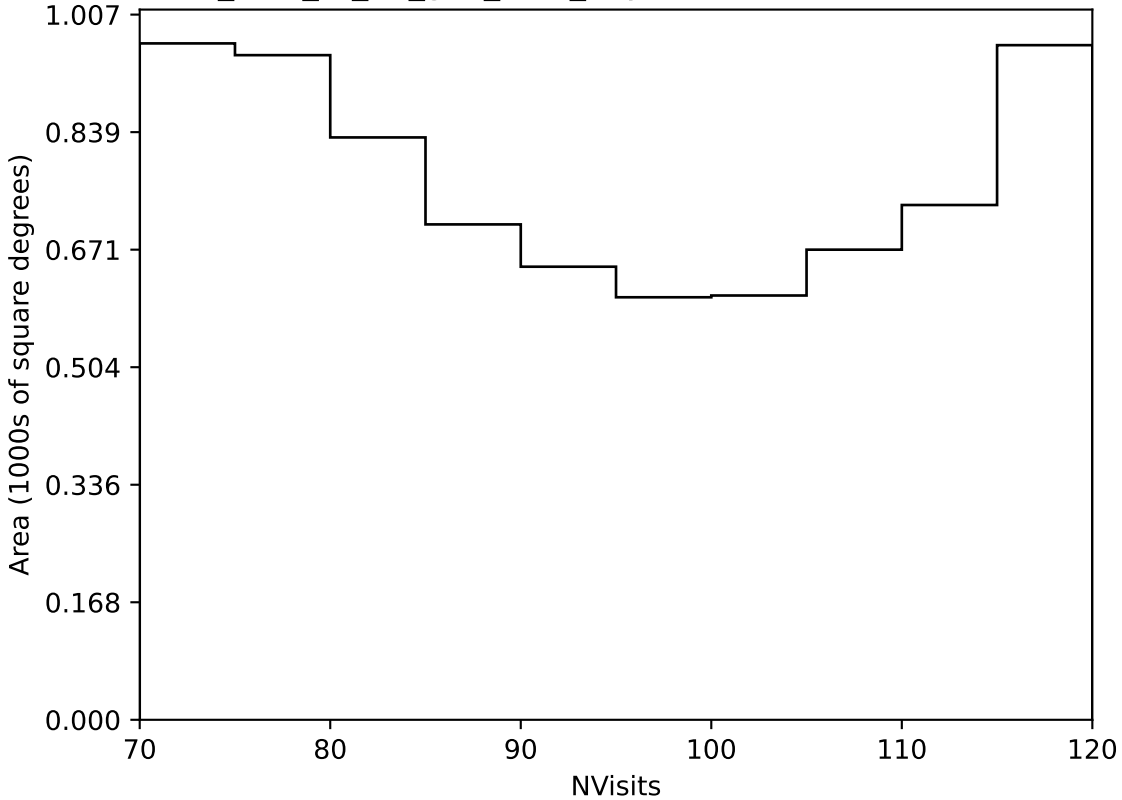
too_elab_r8_d2_griz_v3.4_10yrs Yr 3-4 all bands: NVisits
