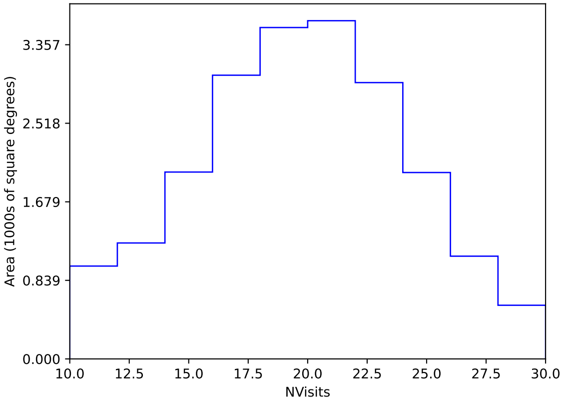
too_elab_r8_d2_griz_v3.4_10yrs Yr 1 y band: NVisits
