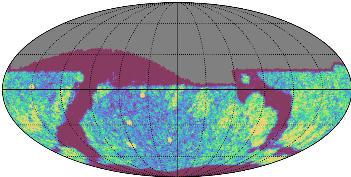
too_elab_r8_d2_griz_v3.4_10yrs Yr 1 r band: NVisits
