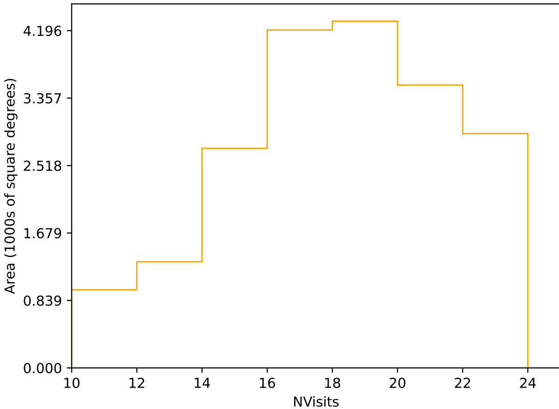
too_elab_r8_d2_griz_v3.4_10yrs Yr 1 r band: NVisits
