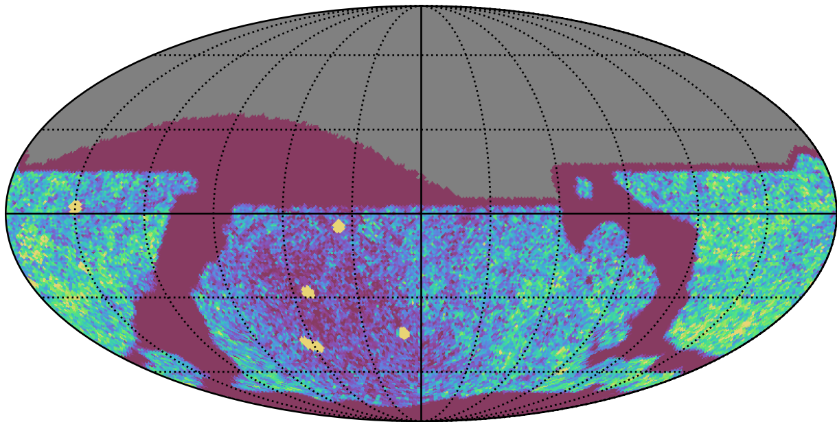
too_elab_r8_d2_griz_v3.4_10yrs Yr 1 all bands: NVisits
