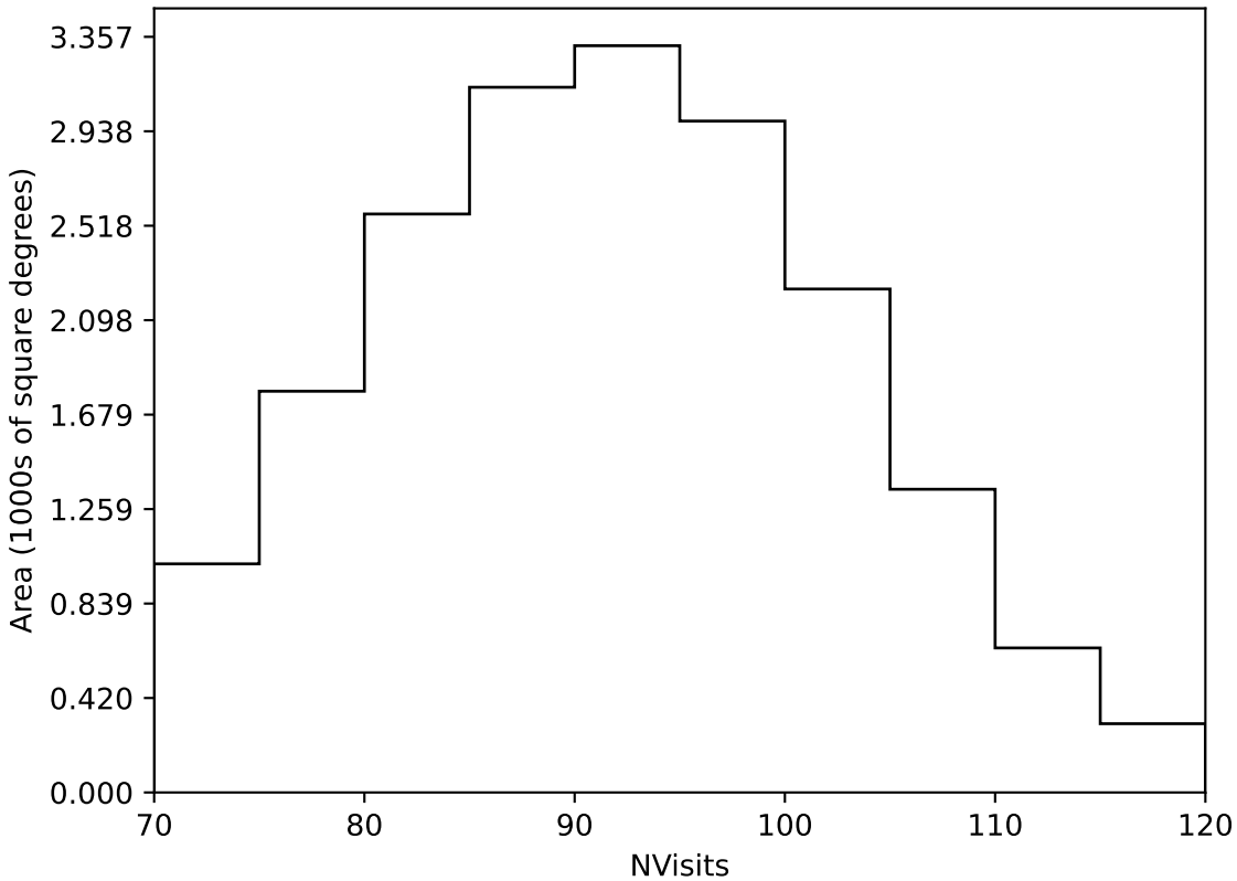
too_elab_r8_d2_griz_v3.4_10yrs Yr 1 all bands: NVisits
