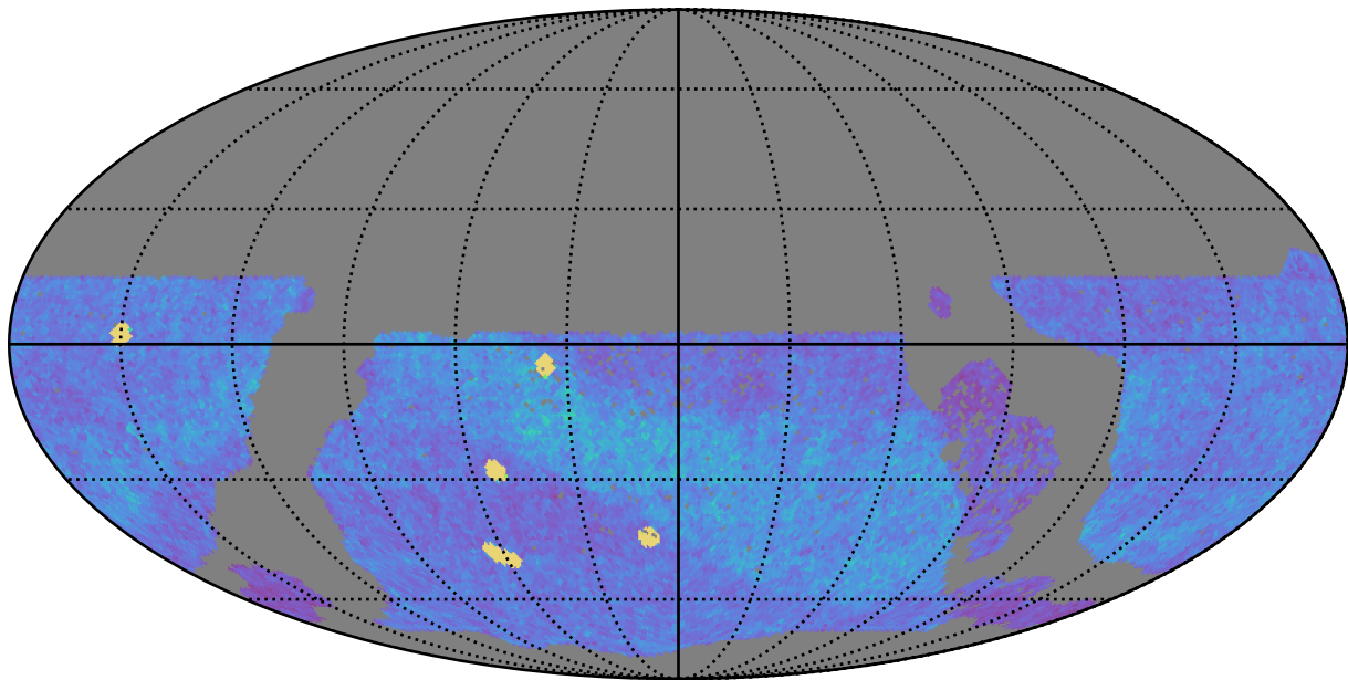
too_elab_r8_d2_griz_v3.4_10yrs WFD z band: NVisits
