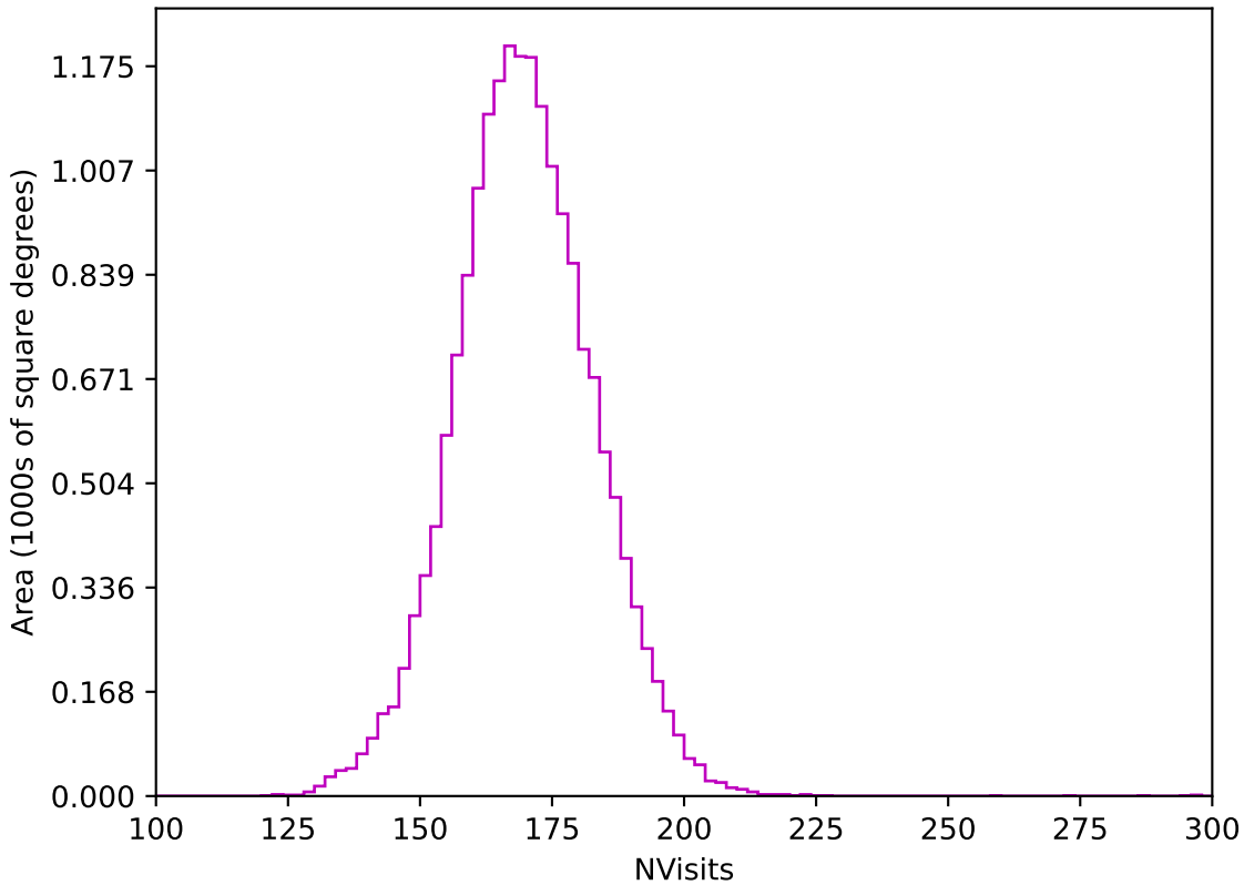
too_elab_r8_d2_griz_v3.4_10yrs WFD z band: NVisits
