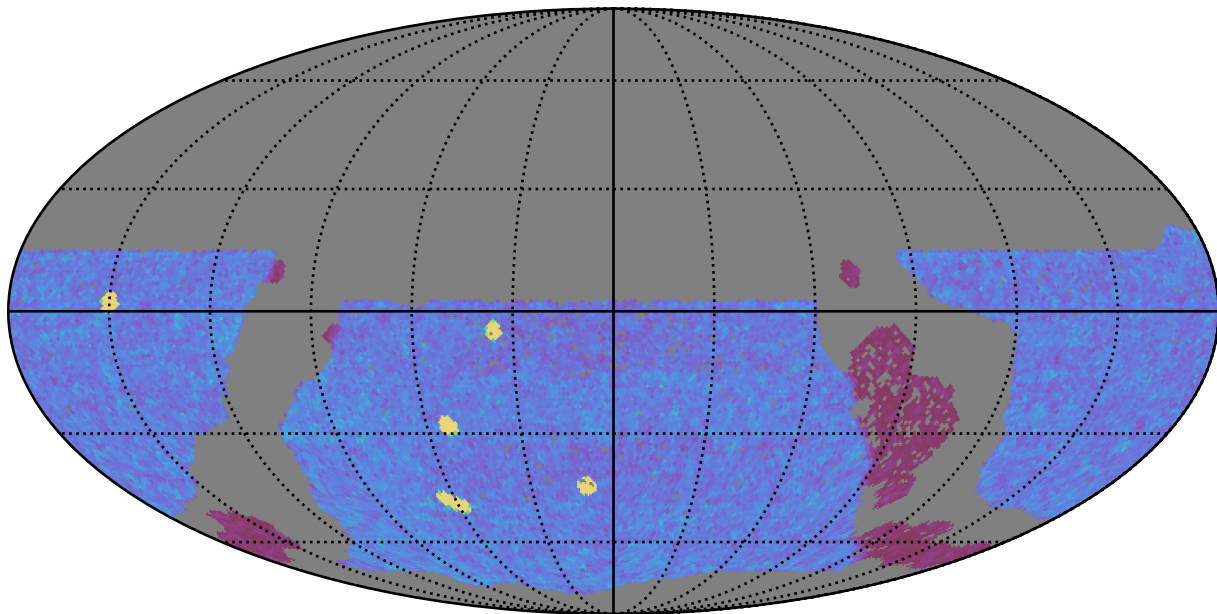
too_elab_r8_d2_griz_v3.4_10yrs WFD y band: NVisits
