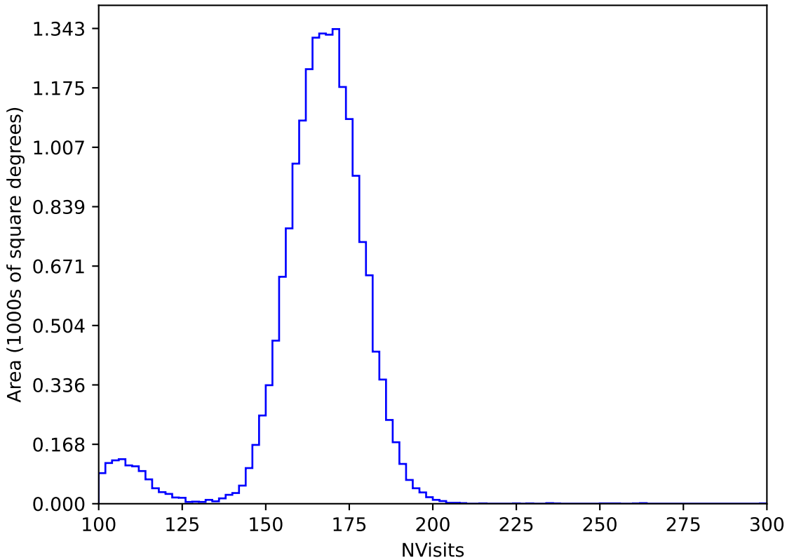
too_elab_r8_d2_griz_v3.4_10yrs WFD y band: NVisits
