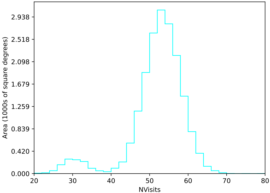
too_elab_r8_d2_griz_v3.4_10yrs WFD u band: NVisits
