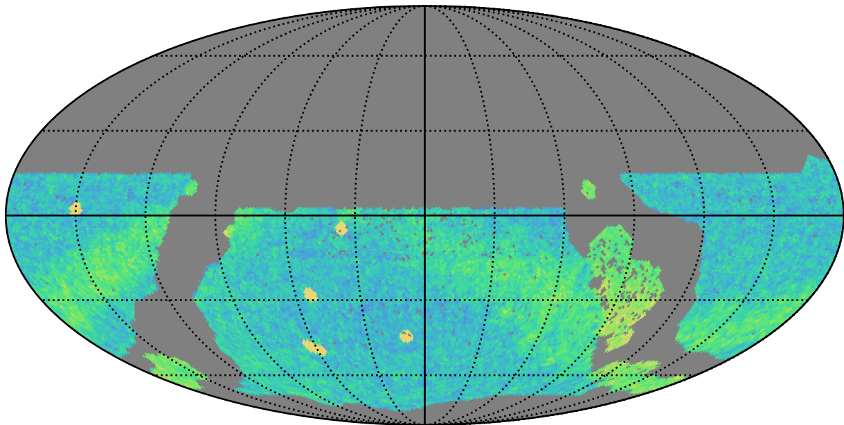
too_elab_r8_d2_griz_v3.4_10yrs WFD r band: NVisits
