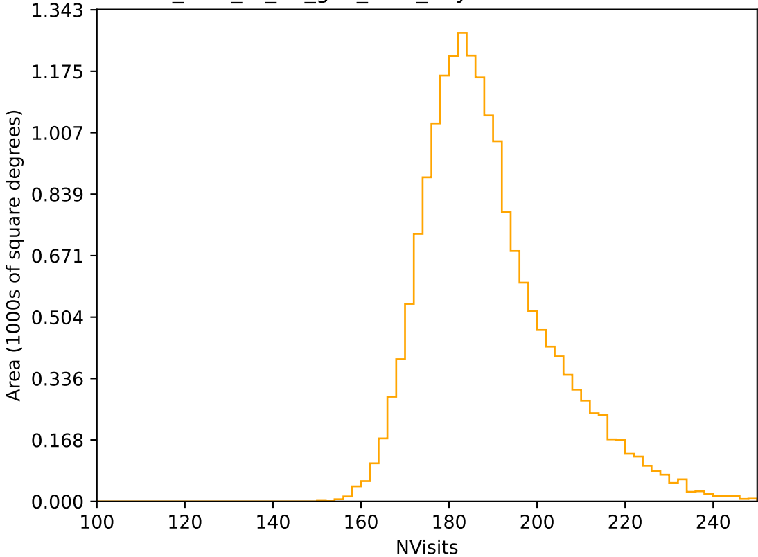
too_elab_r8_d2_griz_v3.4_10yrs WFD r band: NVisits
