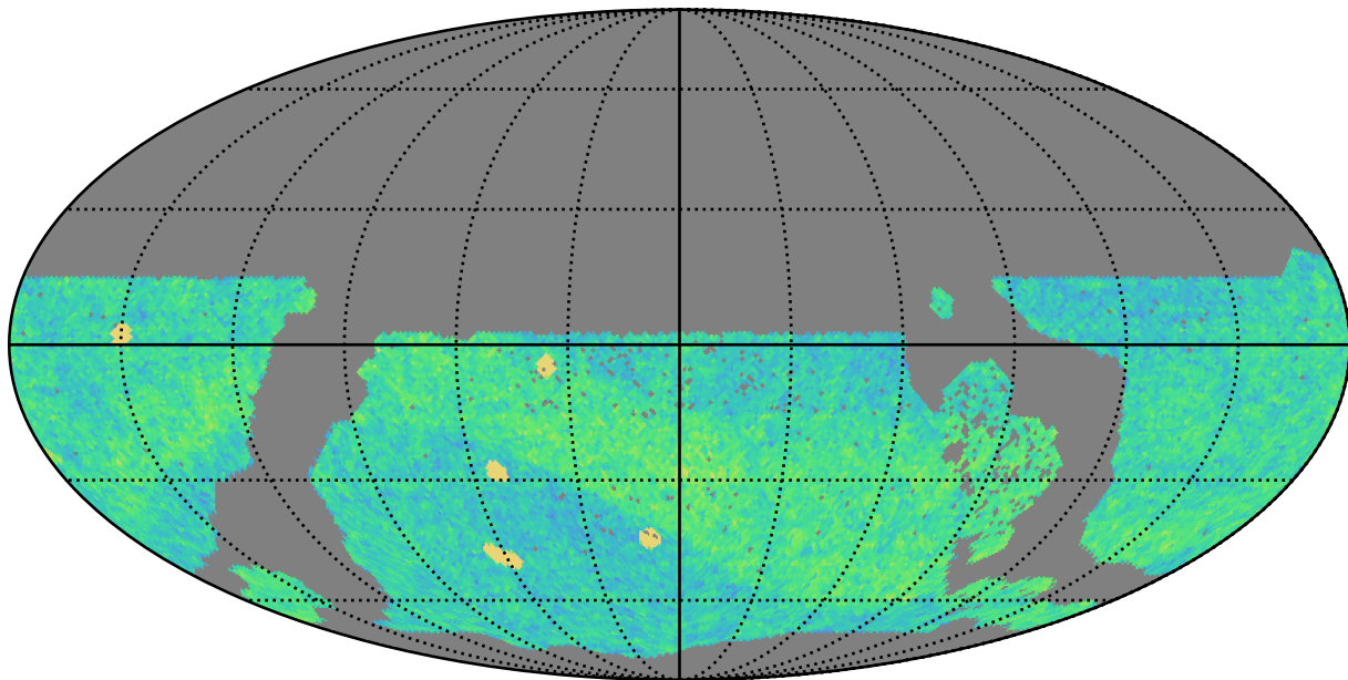
too_elab_r8_d2_griz_v3.4_10yrs WFD i band: NVisits
