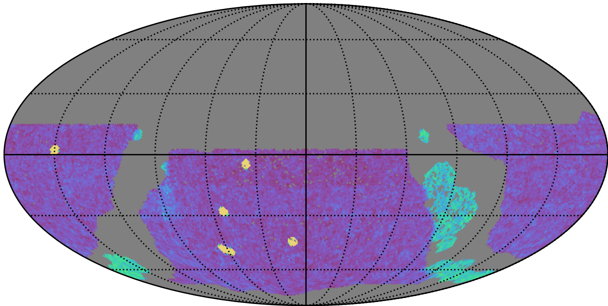
too_elab_r8_d2_griz_v3.4_10yrs WFD g band: NVisits
