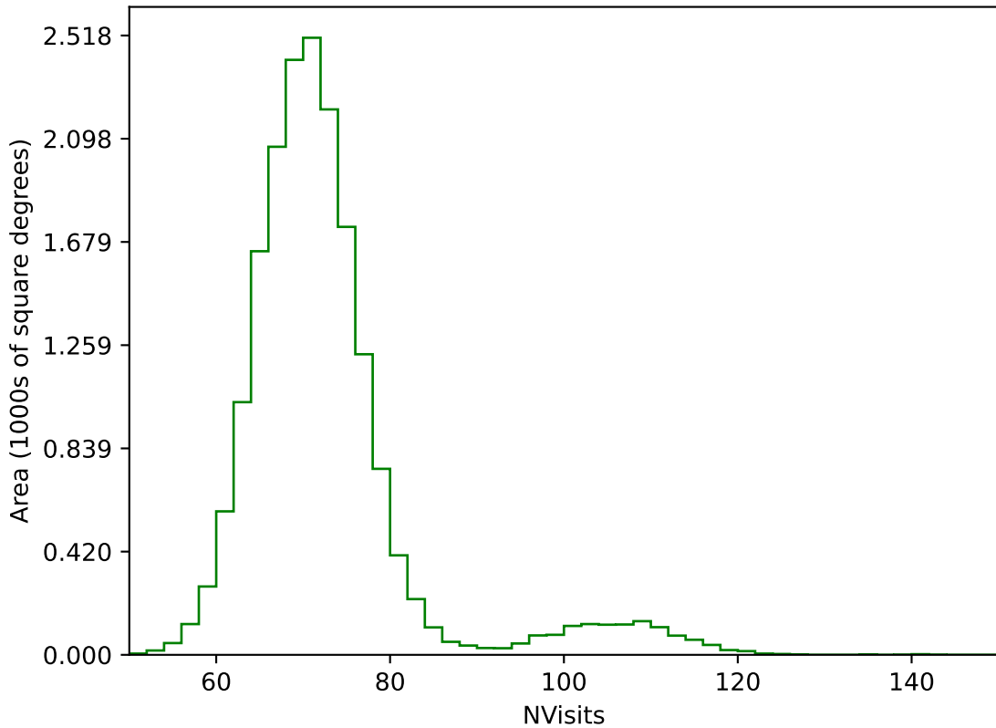
too_elab_r8_d2_griz_v3.4_10yrs WFD g band: NVisits
