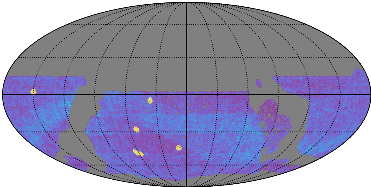
too_elab_r8_d2_griz_v3.4_10yrs WFD all bands: NVisits
