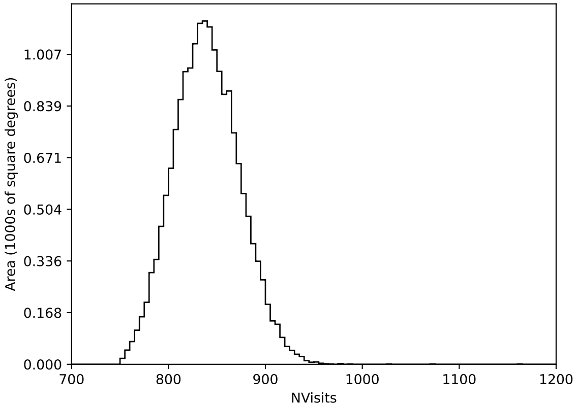
too_elab_r8_d2_griz_v3.4_10yrs WFD all bands: NVisits
