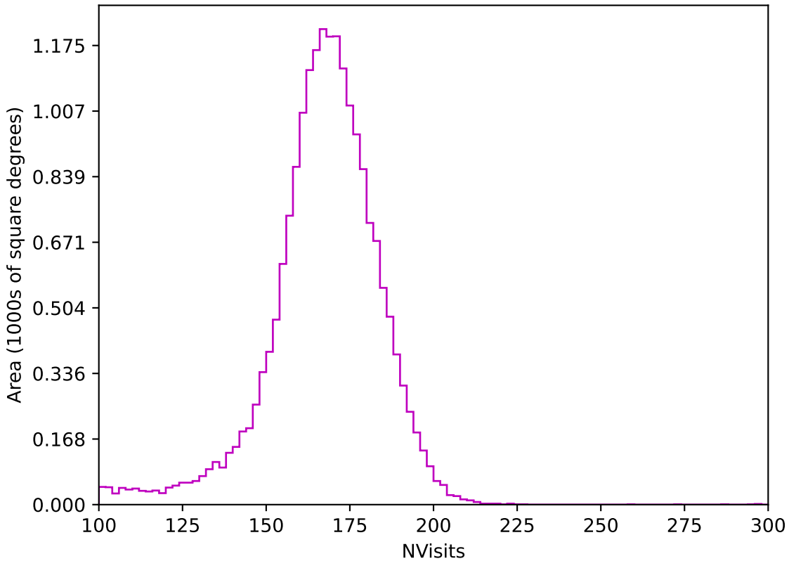
too_elab_r8_d2_griz_v3.4_10yrs All sky z band: NVisits
