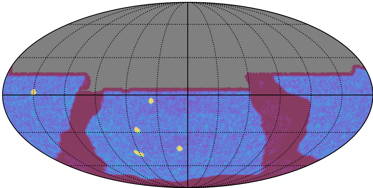
too_elab_r8_d2_griz_v3.4_10yrs All sky y band: NVisits
