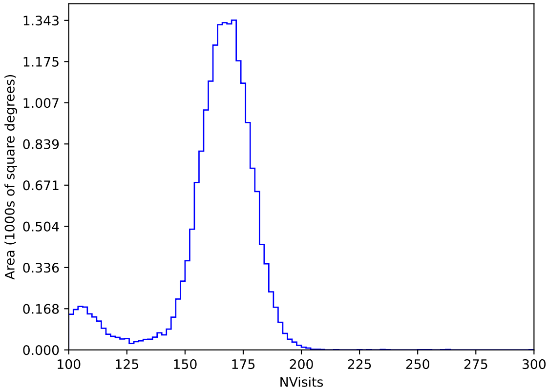
too_elab_r8_d2_griz_v3.4_10yrs All sky y band: NVisits
