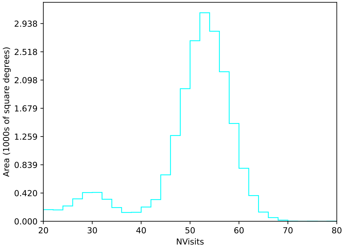
too_elab_r8_d2_griz_v3.4_10yrs All sky u band: NVisits
