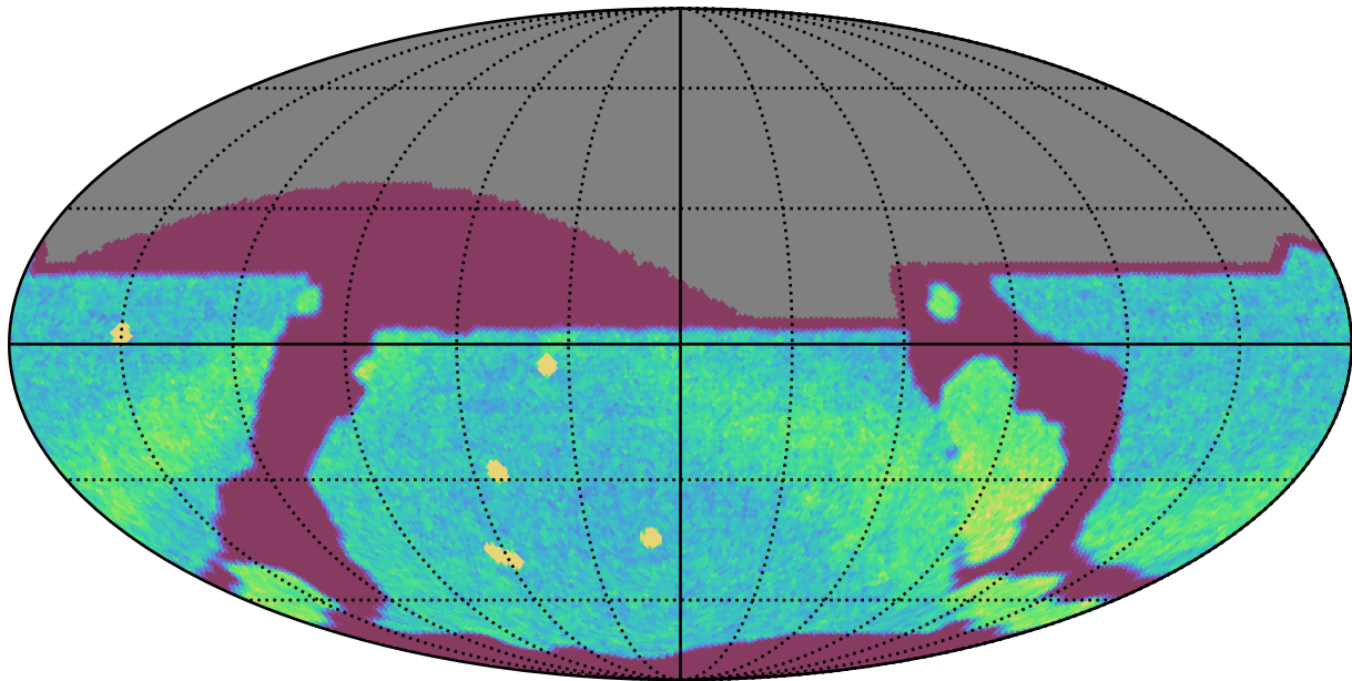
too_elab_r8_d2_griz_v3.4_10yrs All sky r band: NVisits
