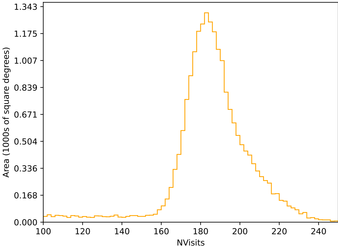
too_elab_r8_d2_griz_v3.4_10yrs All sky r band: NVisits
