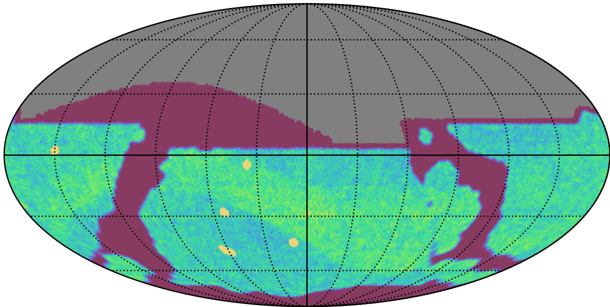
too_elab_r8_d2_griz_v3.4_10yrs All sky i band: NVisits
