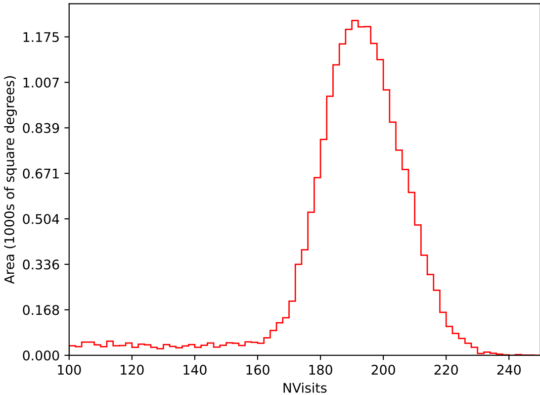
too_elab_r8_d2_griz_v3.4_10yrs All sky i band: NVisits
