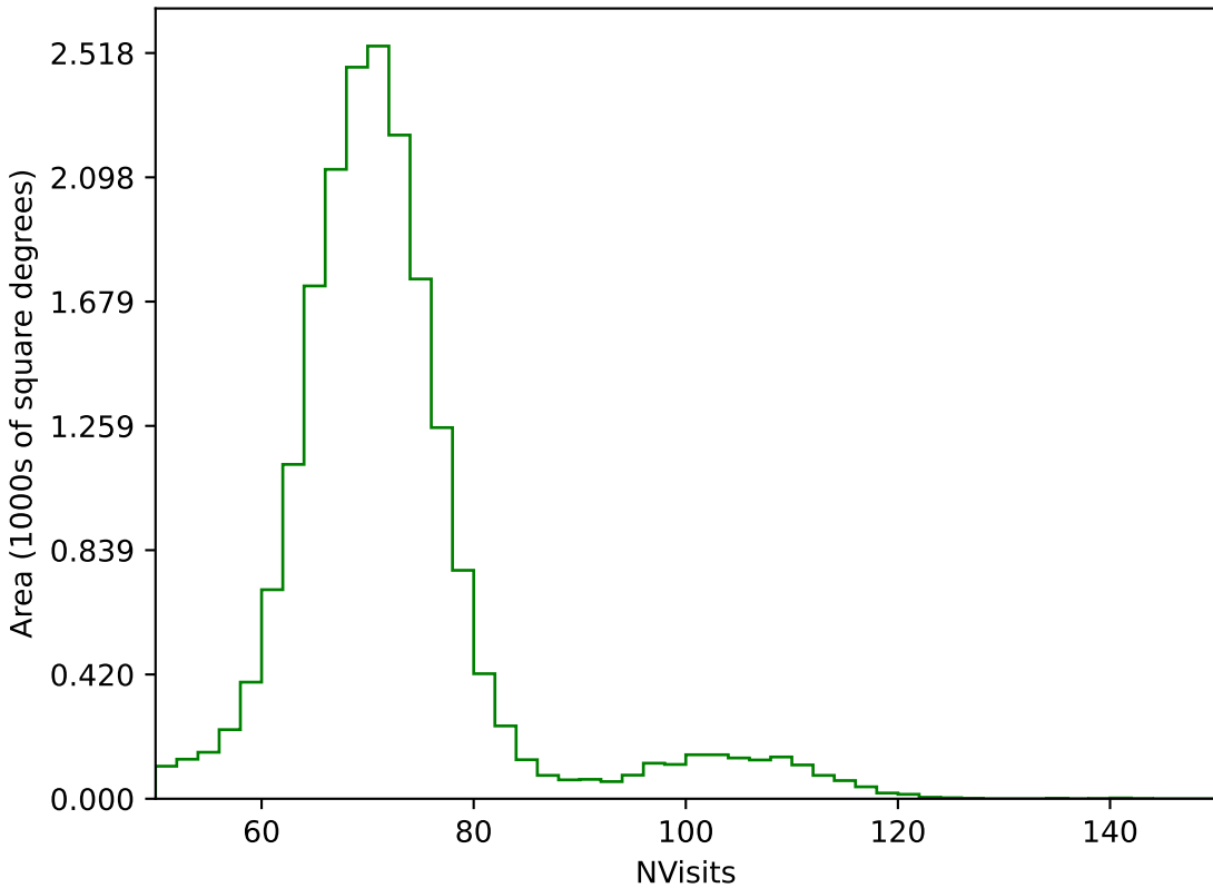
too_elab_r8_d2_griz_v3.4_10yrs All sky g band: NVisits
