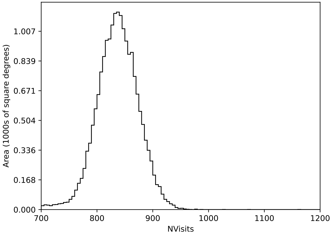
too_elab_r8_d2_griz_v3.4_10yrs All sky all bands: NVisits
