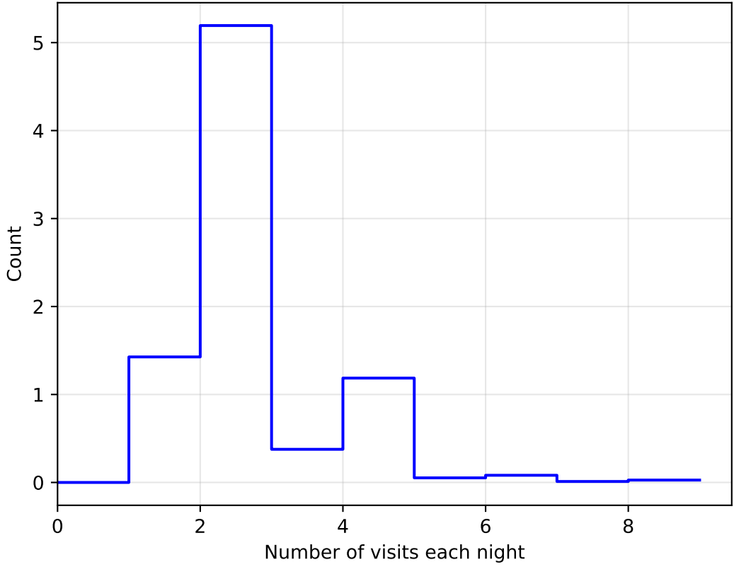
too_elab_r8_d2_griz_v3.4_10yrs WFD: NVisitsPerNight
