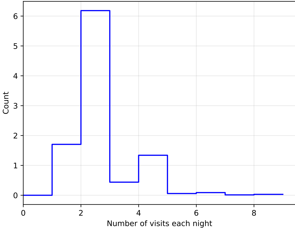
too_elab_r8_d2_griz_v3.4_10yrs All sky: NVisitsPerNight
