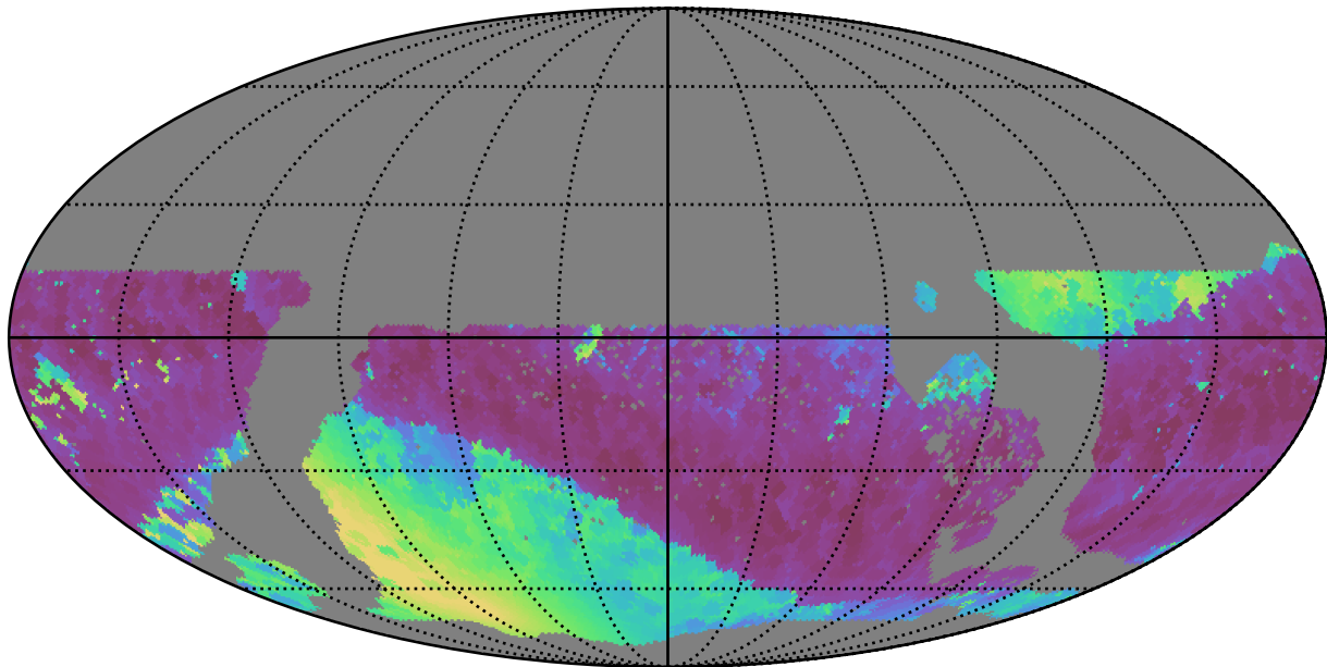
too_elab_r8_d2_griz_v3.4_10yrs WFD z band: Min solarElong
