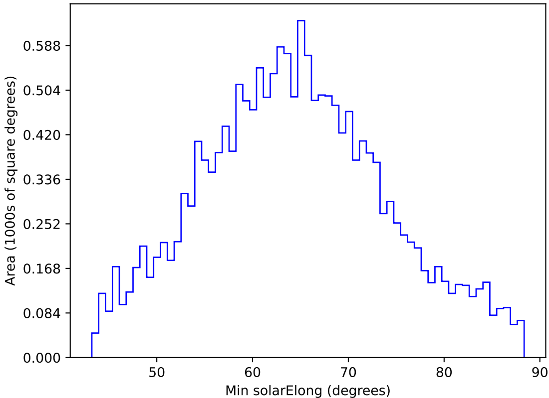
too_elab_r8_d2_griz_v3.4_10yrs WFD y band: Min solarElong
