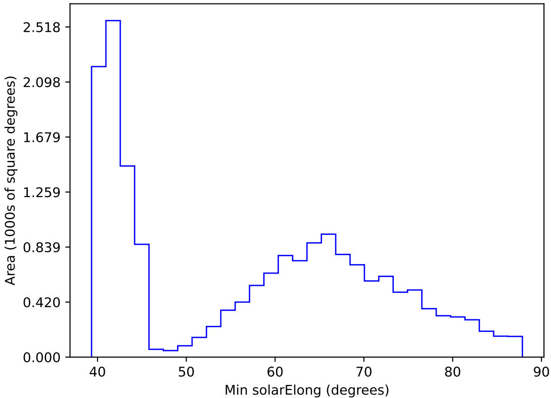
too_elab_r8_d2_griz_v3.4_10yrs WFD r band: Min solarElong
