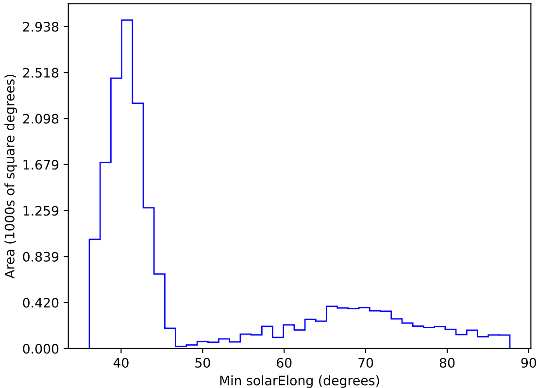
too_elab_r8_d2_griz_v3.4_10yrs WFD i band: Min solarElong
