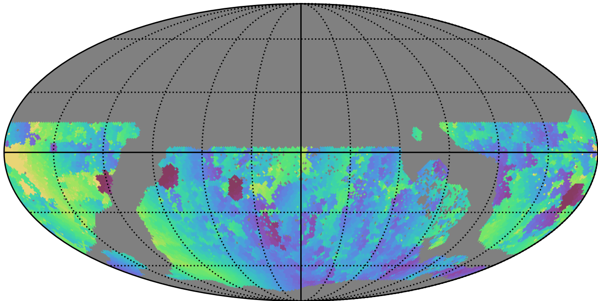
too_elab_r8_d2_griz_v3.4_10yrs WFD g band: Min solarElong
